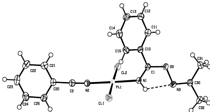
Figure 1. Molecular structure of the mono-iminoacylated Pt II complex trans -[PtCl 2 {NH=C(Ph)ON=CMe 2 }(NCPH)] ( 5c ) with the atomic numbering scheme (ellipsoids are drawn at 50% probability).
