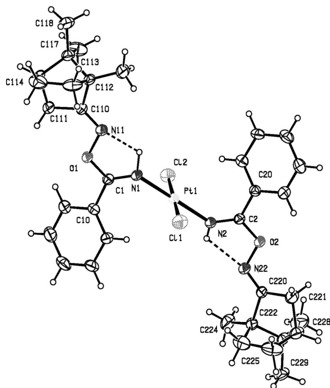
Figure 2. Molecular structure of the iminoacylated Pt II complex trans -[PtCl 2 {NH=C(Ph)ON=C(C 9 H 16 )} 2 ] ( 7b ) with the atomic numbering scheme (ellipsoids are drawn at 50% probability).
